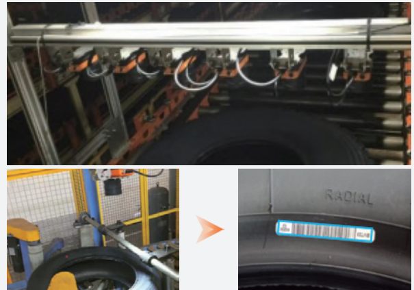
Full view tyre code reading
