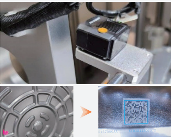
High-speed reading of distorted reflective and low-contrast codes on ECU cover
