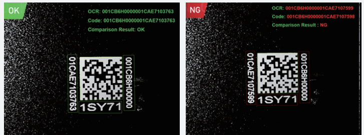
Inkjet interference in lithium battery information detection
