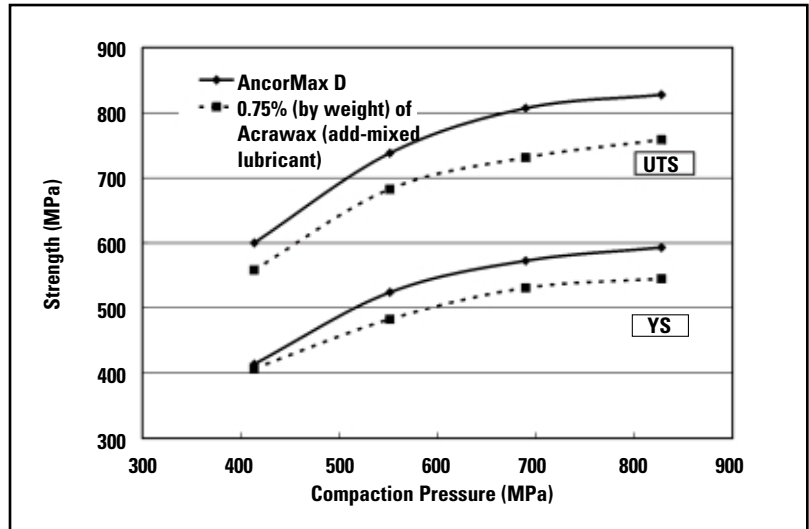
Figure 3—Strength of FLN2-4405 sintered at 1,260°C (2,300°F).
