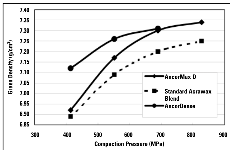
Figure 1—Comparison of the compressibility of a regular premix with AncorDense and AncorMax D.
