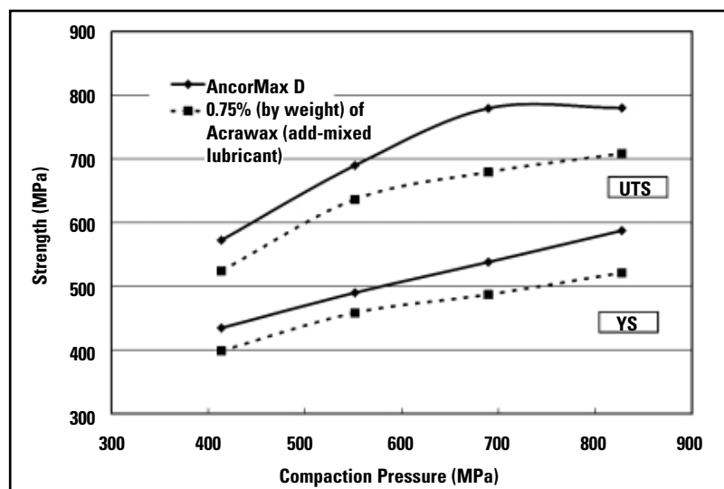
Figure 2—Strength of FLN2-4405 sintered at 1,120°C (2,050°F).
