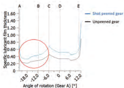
Figure 11—Comparison of specific lubricant film thickness.
