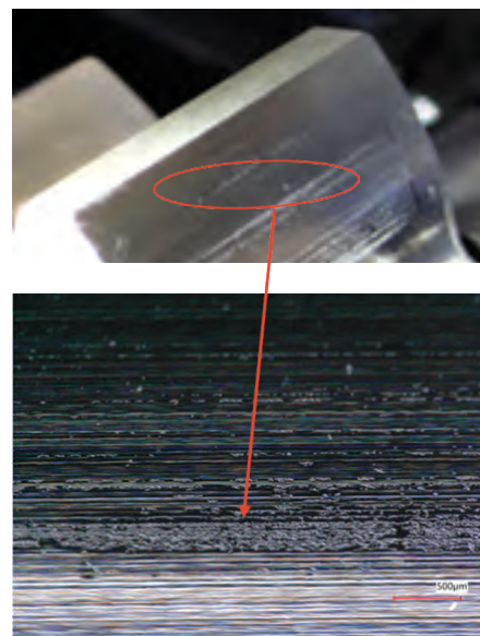
Figure 12—Micropitting safety on the path of contact of gears according to ISO 6336-22:2018.
