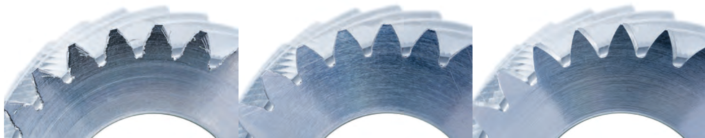
Gear hobbled with remaining hob burr (left). Gear hobbled and rough deburred during hobbing (middle). Gear after hobbing, rough deburring and then chamfer hobbing in parallel with hobbing (right).
