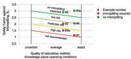
Figure 7—Micropitting safety factor according to Ref. 18.
