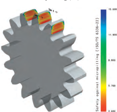
Figure 13—Safety against micropitting on the tooth.
