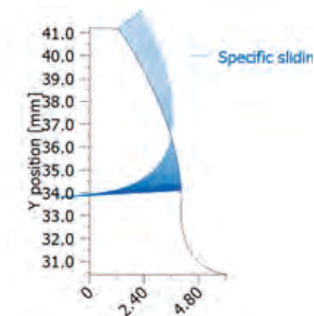
Figure 8—Specific sliding along tooth profile.
