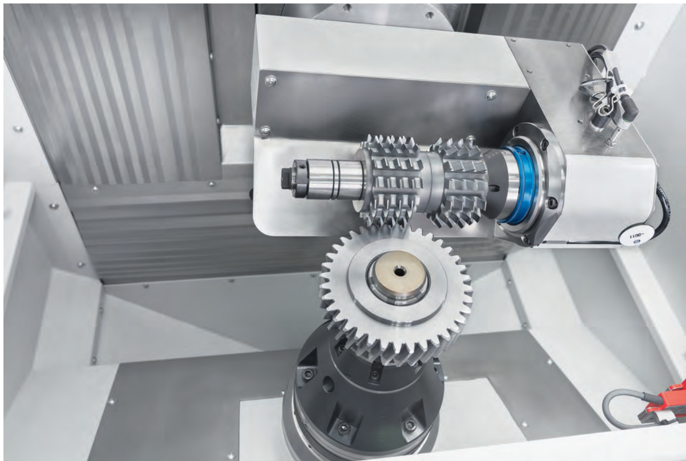
Chamfer hobbing with low tool cost.
