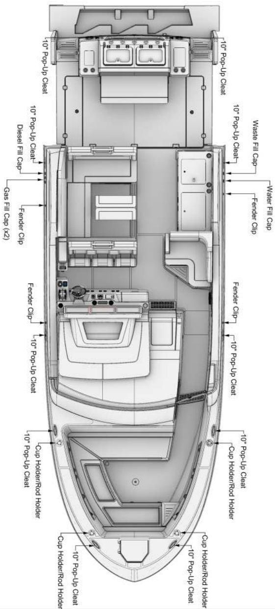
FX Deck Hardware Top View
