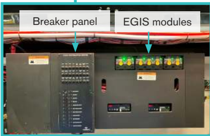
Battery management box
