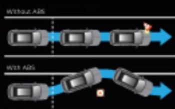
Anti-lock Braking System (ABS)
