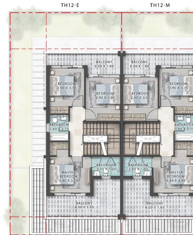
FIRST FLOOR
