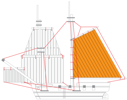
BRIGANTINE SAIL CUT-OUT
