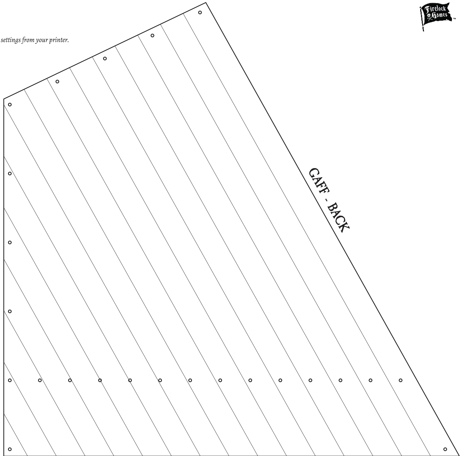
BRIGANTINE SAIL CUT-OUT
