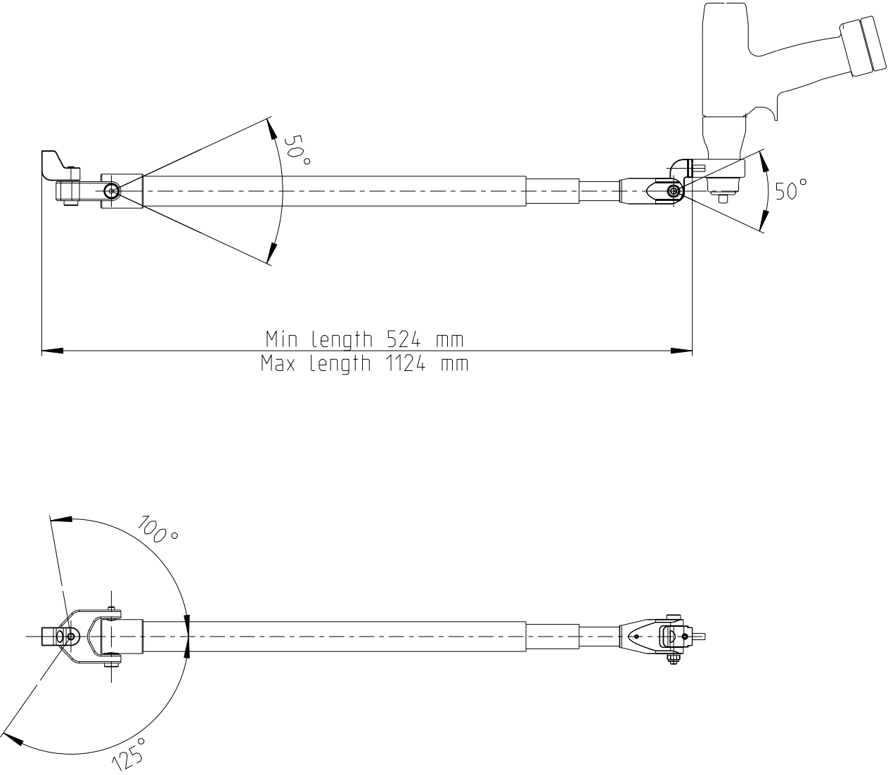
BENCH STAND
