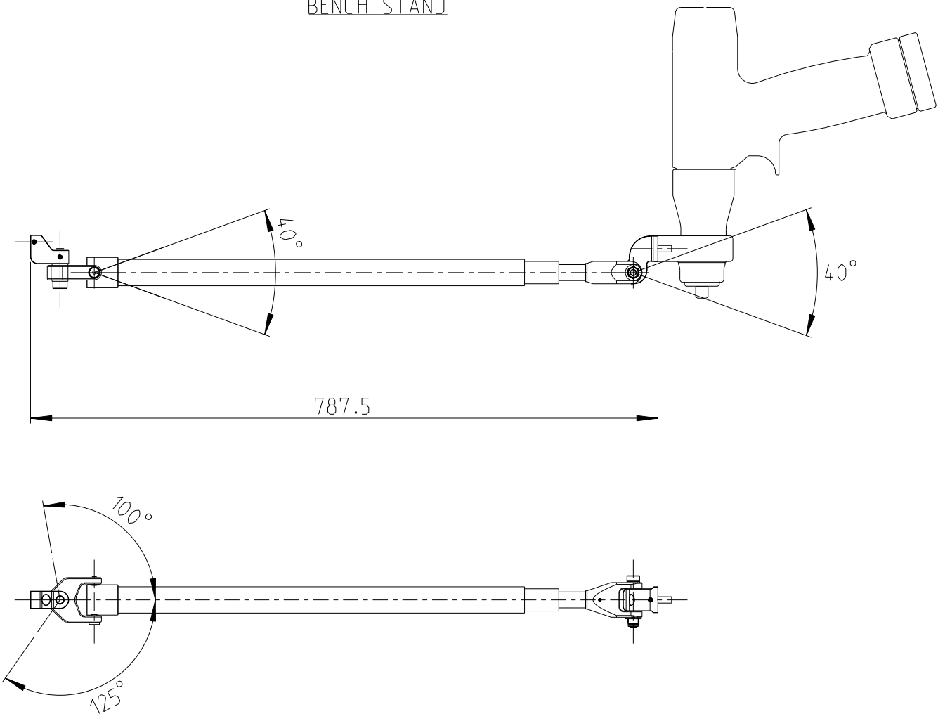
BENCH STAND
