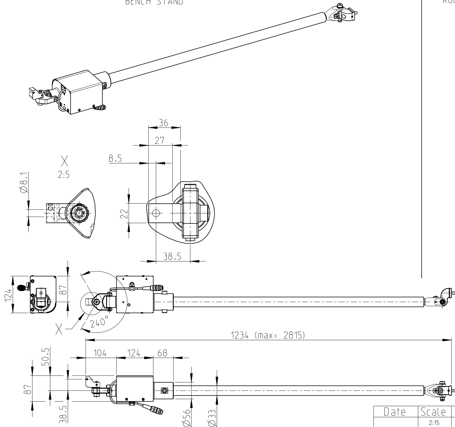
BENCH STAND
