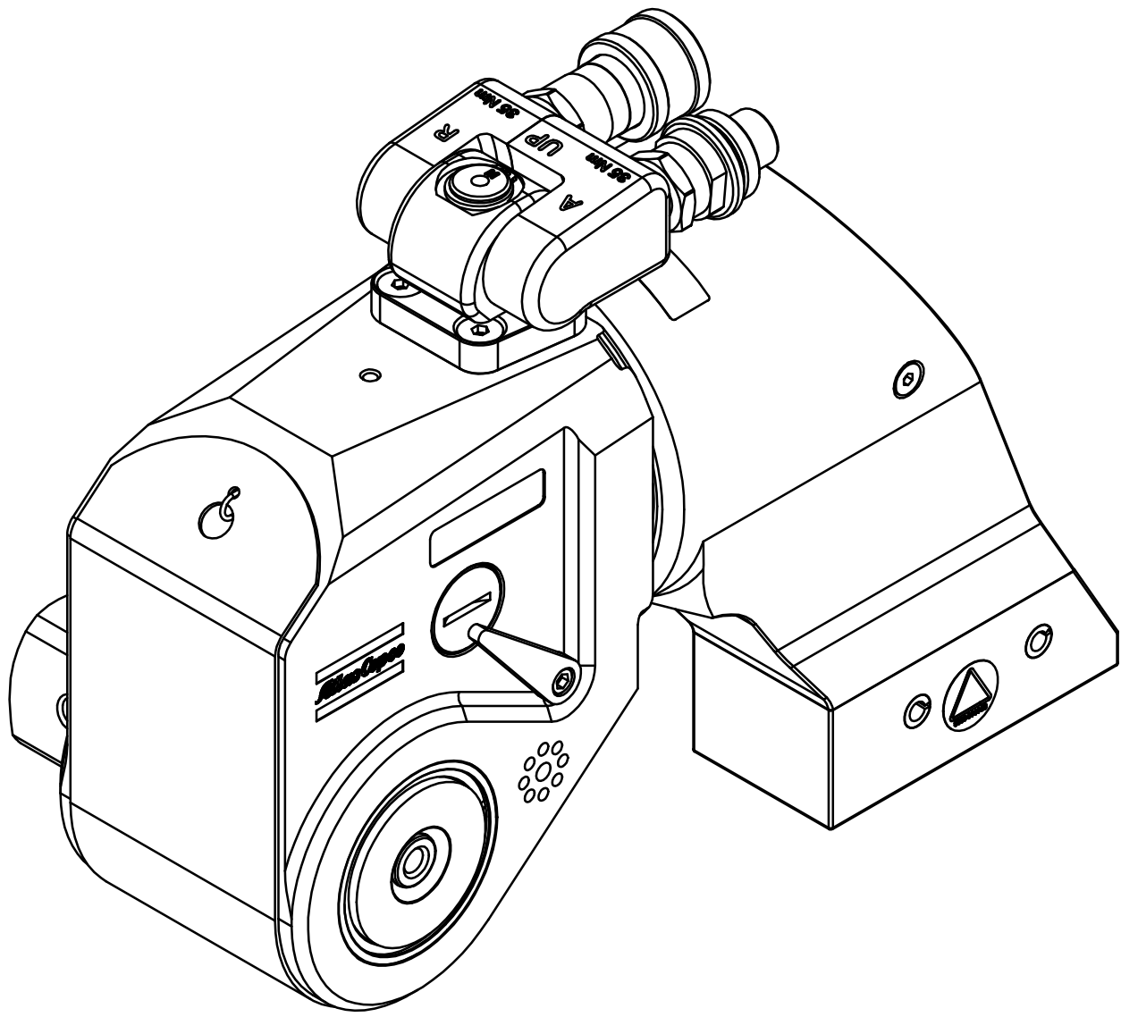
ISOMETRIC VIEW
