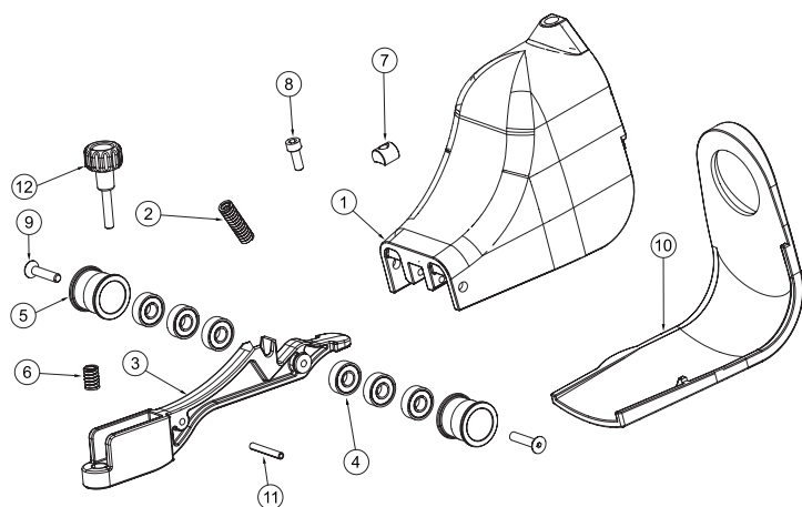
2050545413 Arm support
