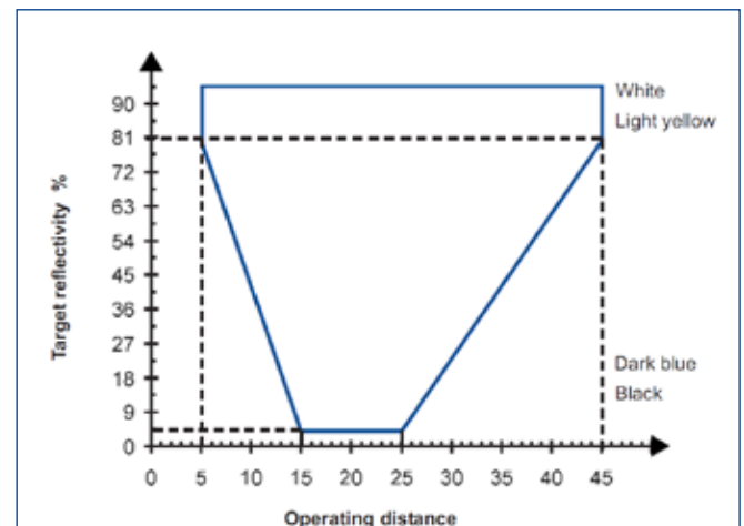
S65-V1: operating distance according to target reflectivity degree
