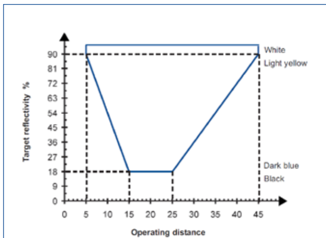
S65-V0: operating distance according to target reflectivity degree
