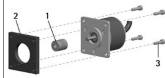
with flange ST-58-FLNG
