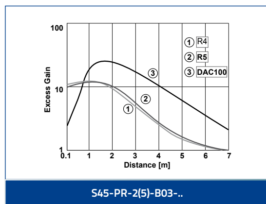
EXCESS GAIN
