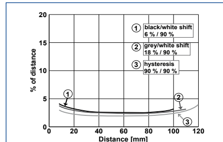
B/W SHIFT
