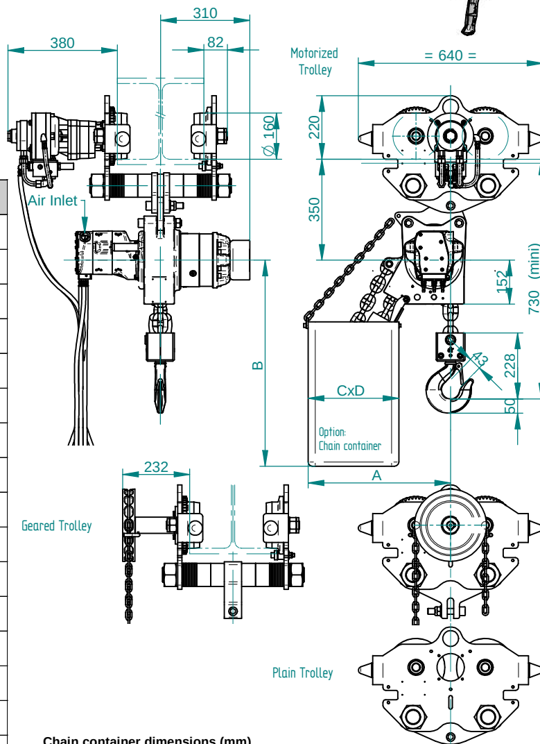
Chain container dimensions (mm)
