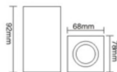
ECWL 302-1 Size:68*92*78MM MR16
