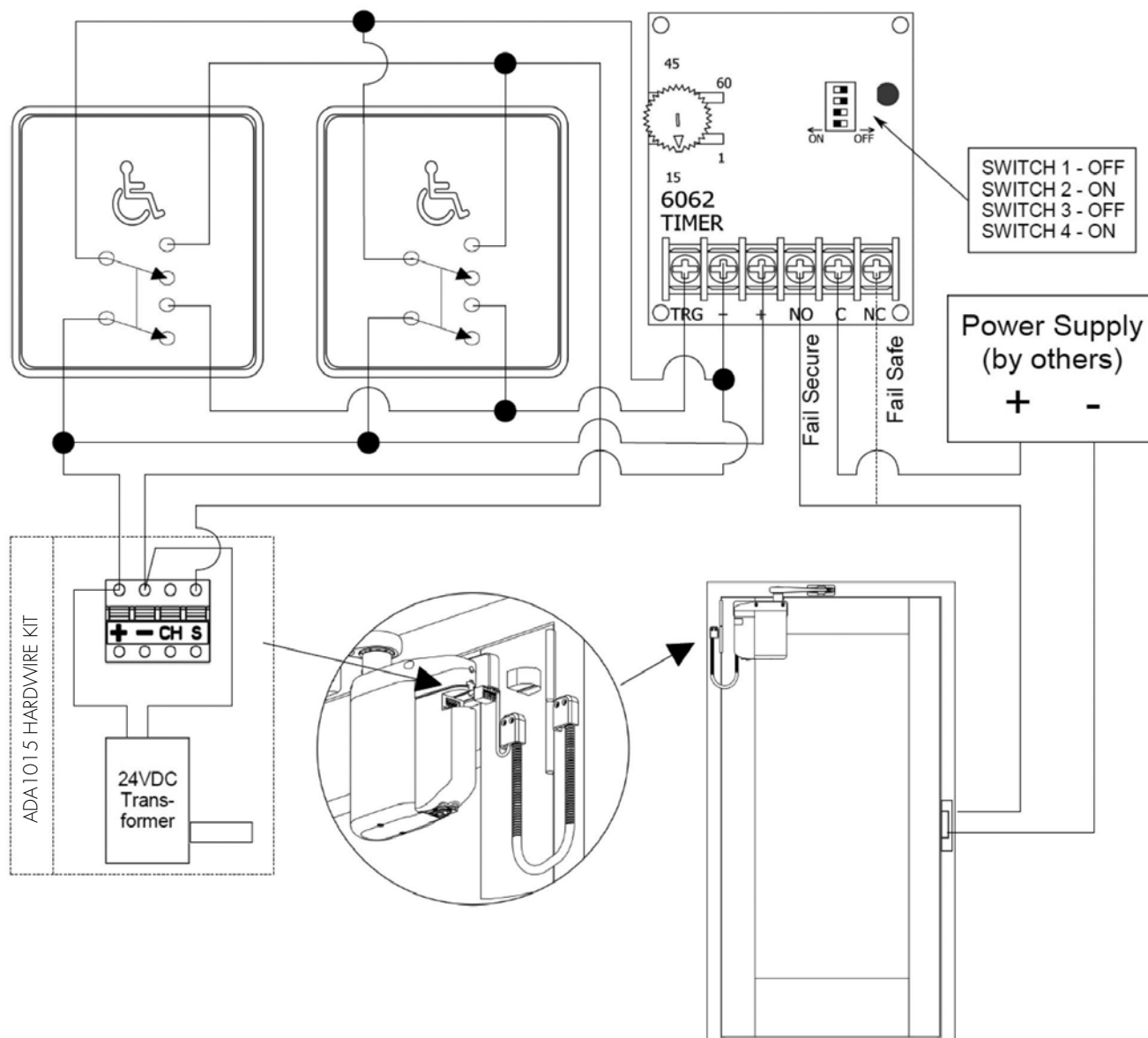
Hardwired Pushbutton Switches
