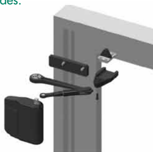
Operator Push Side – Parallel Arm
