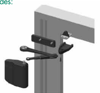
Operator Push Side - Parallel Arm (illustrated) or Pull Side - Regular Arm
