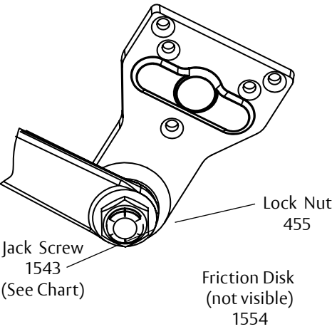
Hold Open Arms Only
