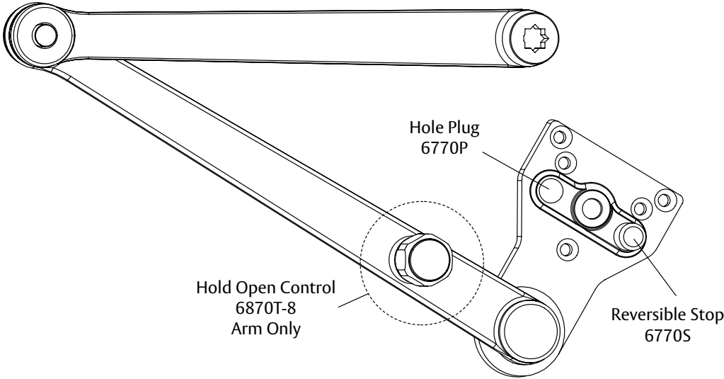
Hold Open Arm Shown (CLP-T)
