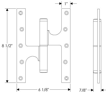
PHNG8.5x6.125 Paumelle Hinge, 7/8" barrel 8 1/2" x 6 1/8" / Each . . . . . $ 445.00
