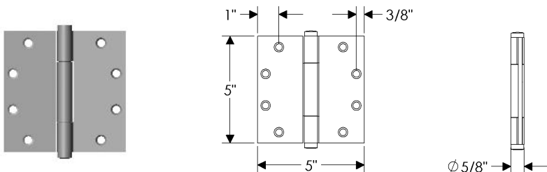
HNG5A Concealed Bearing Hinge 5" x 5" / Each ..... $ 214.00
