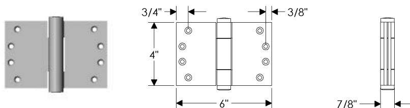
HNGWT4x6 Concealed Bearing Hinge 4" x 6" / Each ..... $ 218.00
