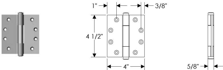
HNG4.5x4A Concealed Bearing Hinge 4 1/2" x 4" / Each ..... $ 204.00
