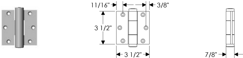
HNG3.5 Concealed Bearing Hinge 3 1/2" x 3 1/2" / Each ..... $ 196.00
