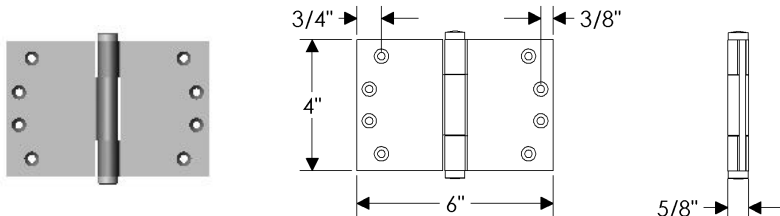
HNGWT4x6A Concealed Bearing Hinge 4" x 6" / Each ..... $ 218.00
