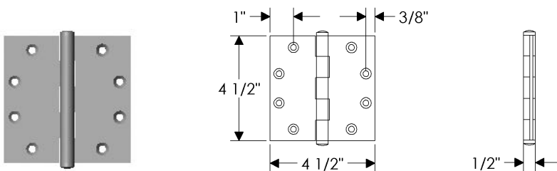
HNG4.5B Plain Bearing Extruded Hinge 4 1/2" x 4 1/2" / Each ..... $ 143.00 • Builders Series Hinge
