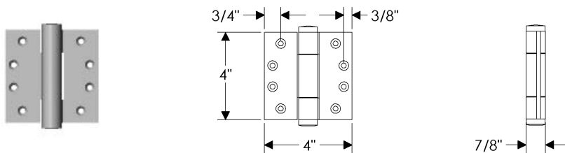
HNG4 Concealed Bearing Hinge 4" x 4" / Each ..... $ 200.00
