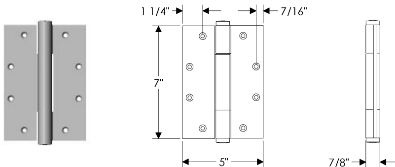
HNG7x5 Concealed Bearing Hinge
