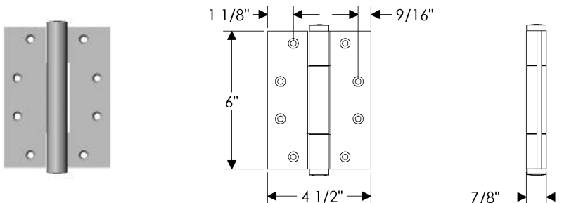
HNG6x4.5 Concealed Bearing Hinge 6" x 4 1/2" / Each ..... $ 234.00 • Hinge leaf thickness is .2
