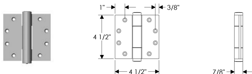
HNG4.5 Concealed Bearing Hinge 4 1/2" x 4 1/2" / Each ..... $ 208.00
