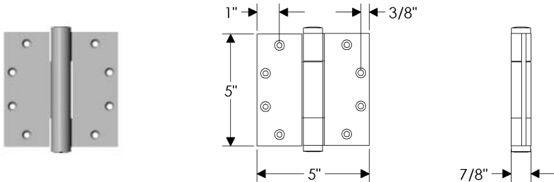
HNG5 Concealed Bearing Hinge 5" x 5" / Each ..... $ 214.00
