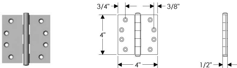
HNG4B Plain Bearing Extruded Hinge 4" x 4" / Each ..... $ 130.00 • Builders Series Hinge
