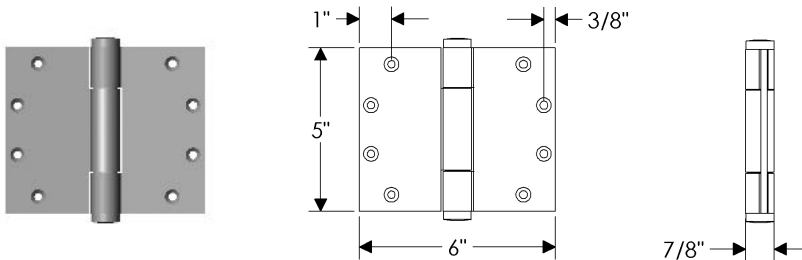
HNGWT5x6 Concealed Bearing Hinge 5" x 6" / Each ..... $ 227.00
