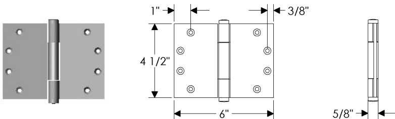
HNGWT4.5x6A Concealed Bearing Hinge 4 1/2" x 6" / Each ..... $ 234.00
