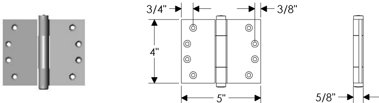
HNGWT4x5A Concealed Bearing Hinge 4" x 5" / Each ..... $ 206.00
