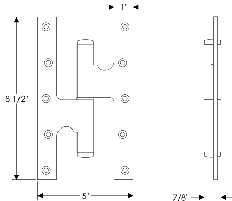
PHNG8.5x5 Paumelle Hinge, 7/8" barrel 8 1/2" x 5" / Each . . . . . $ 424.00
