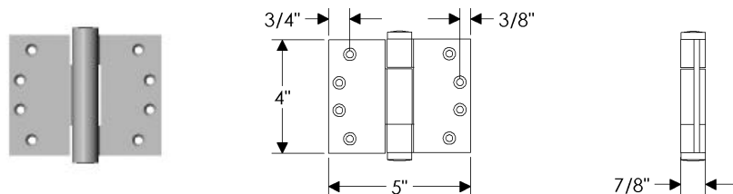
HNGWT4x5 Concealed Bearing Hinge 4" x 5" / Each ..... $ 206.00
