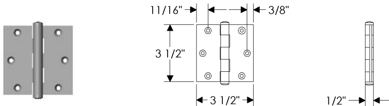
HNG3.5B Plain Bearing Extruded Hinge 3 1/2" x 3 1/2" / Each ..... $ 119.00 • Builders Series Hinge
