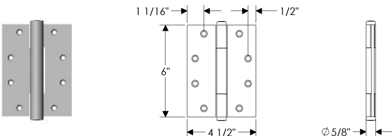
HNG6x4.5A Concealed Bearing Hinge 6" x 4 1/2" / Each ..... $ 234.00
