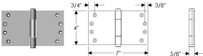
HNGWT4x7A Concealed Bearing Hinge 4" x 7" / Each ..... $ 238.00
