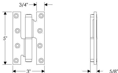
PHNG5x3 Paumelle Hinge, 5/8" barrel 5" x 3" / Each . . . . . $ 182.00
