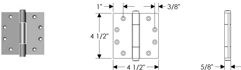
HNG4.5A Concealed Bearing Hinge 4 1/2" x 4 1/2" / Each ..... $ 208.00
