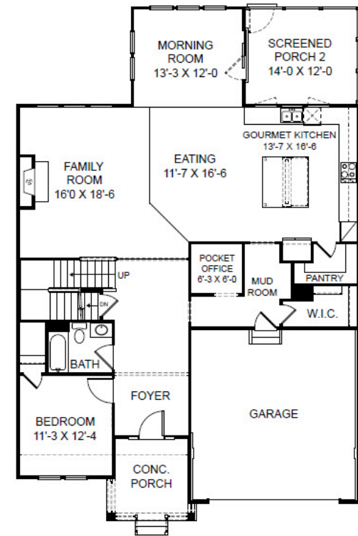
Lower Level Floor Plan
