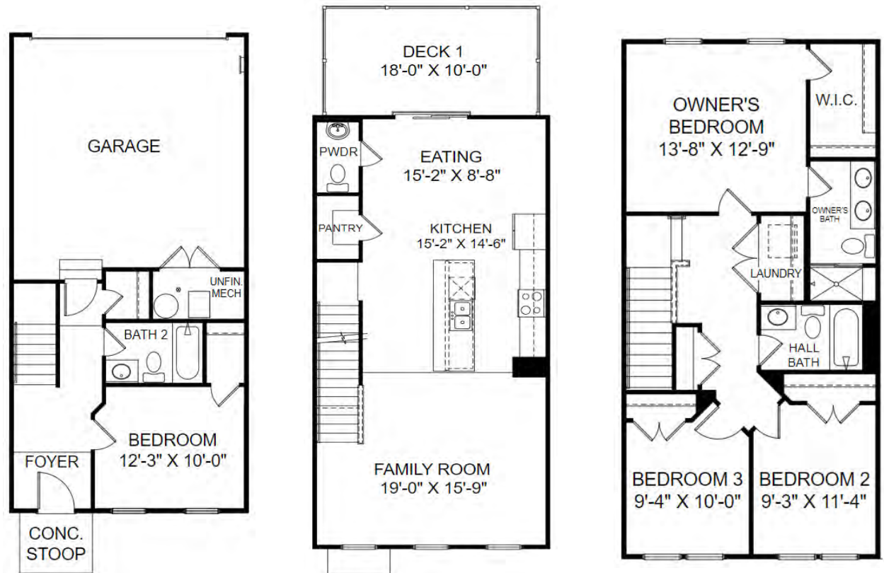
Entry Level Floor Plan
