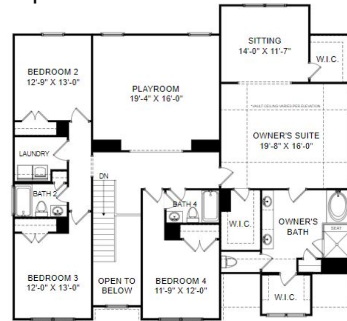
Upper Level Floor Plan
