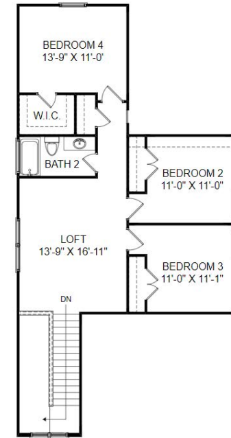
Upper Level floor plan
