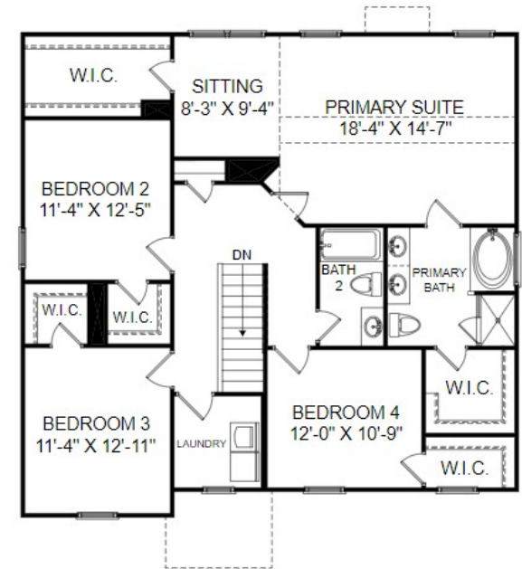
Upper Level Floor Plan
