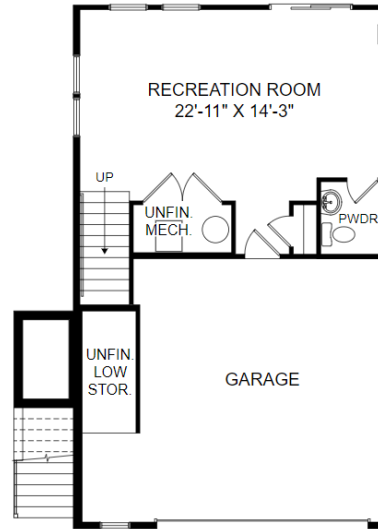
Lower Level Floor Plan
