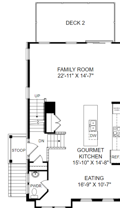
Main Level Floor Plan
