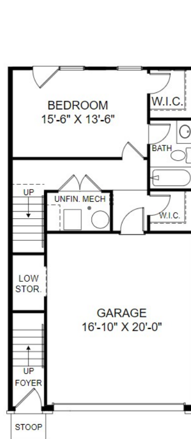
Lower Level Floor Plan
