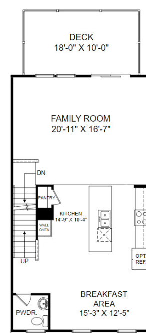
Main Level Floor Plan
