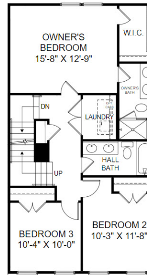
Upper Level Floor Plan
