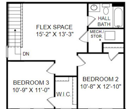
Upper Level Floor Plan
