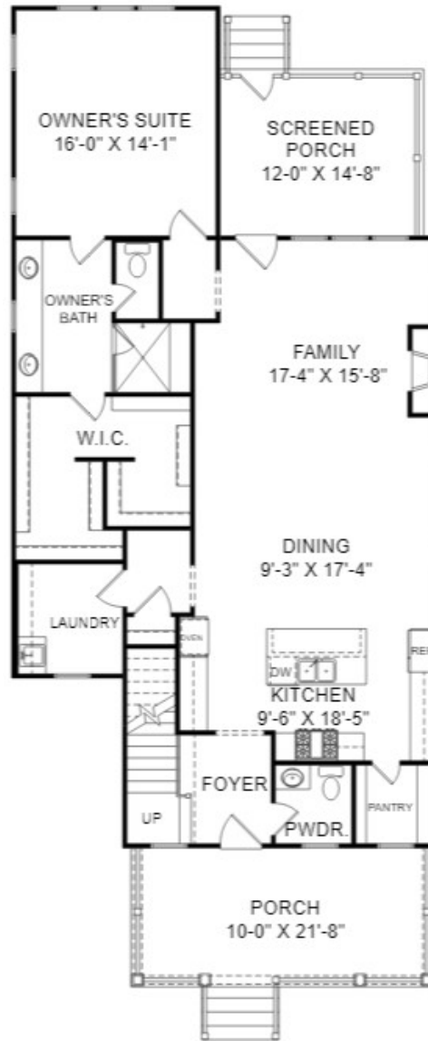
Main Level Floor Plan
