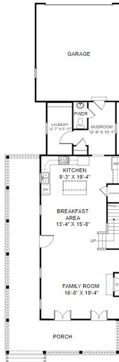
Main Level Floor Plan
