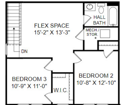
Upper Level Floor Plan
