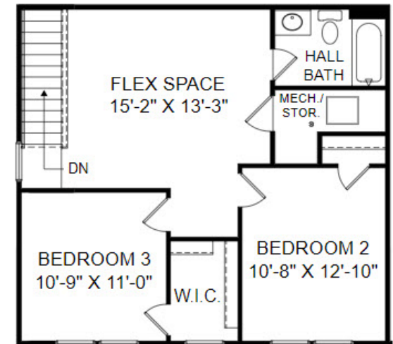
Upper Level Floor Plan
