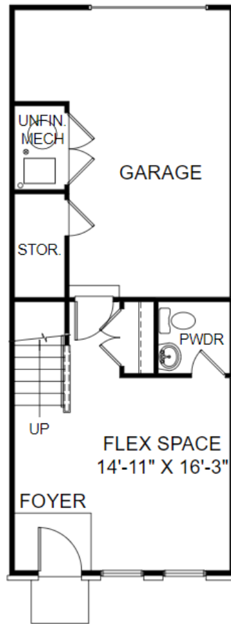
Lower Level Floor Plan
