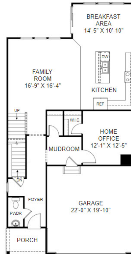
Main Level Floor Plan
