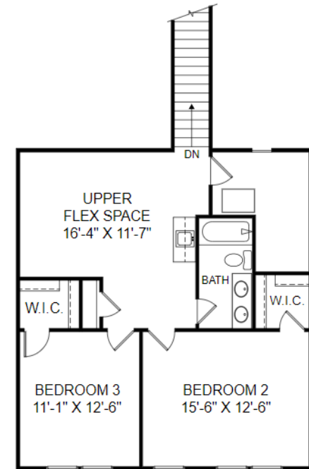
Upper Level Floor Plan
