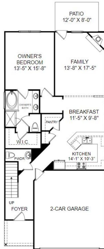
Main Level floor plan
