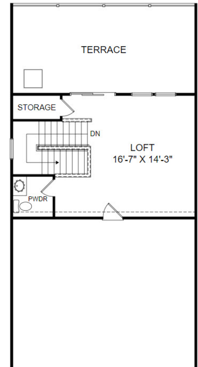
Loft Level Floor Plan
