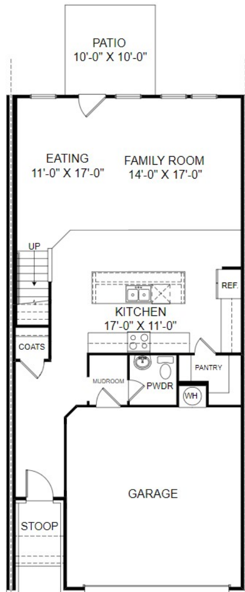
Main Level Floor Plan
