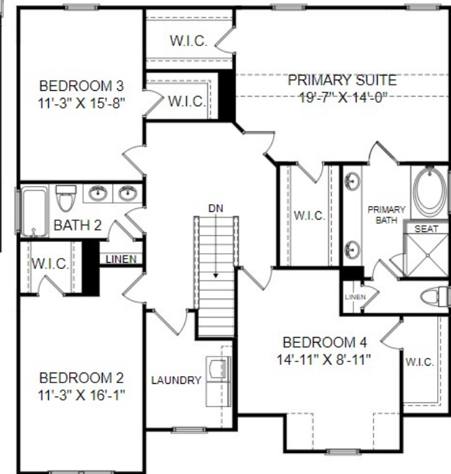
Upper Level Floorplan
