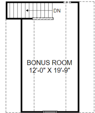
Upper Level Floor Plan
