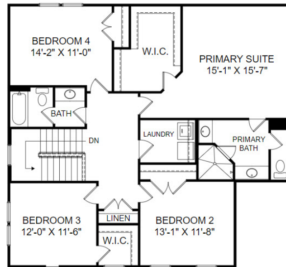
Upper Level Floor Plan
