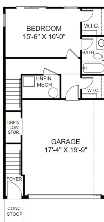
Lower Level Floor Plan
