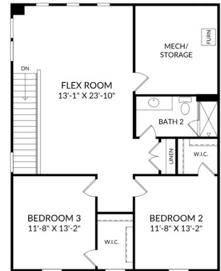
Upper Level Floorplan
