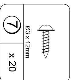
SCREW TCS1048
