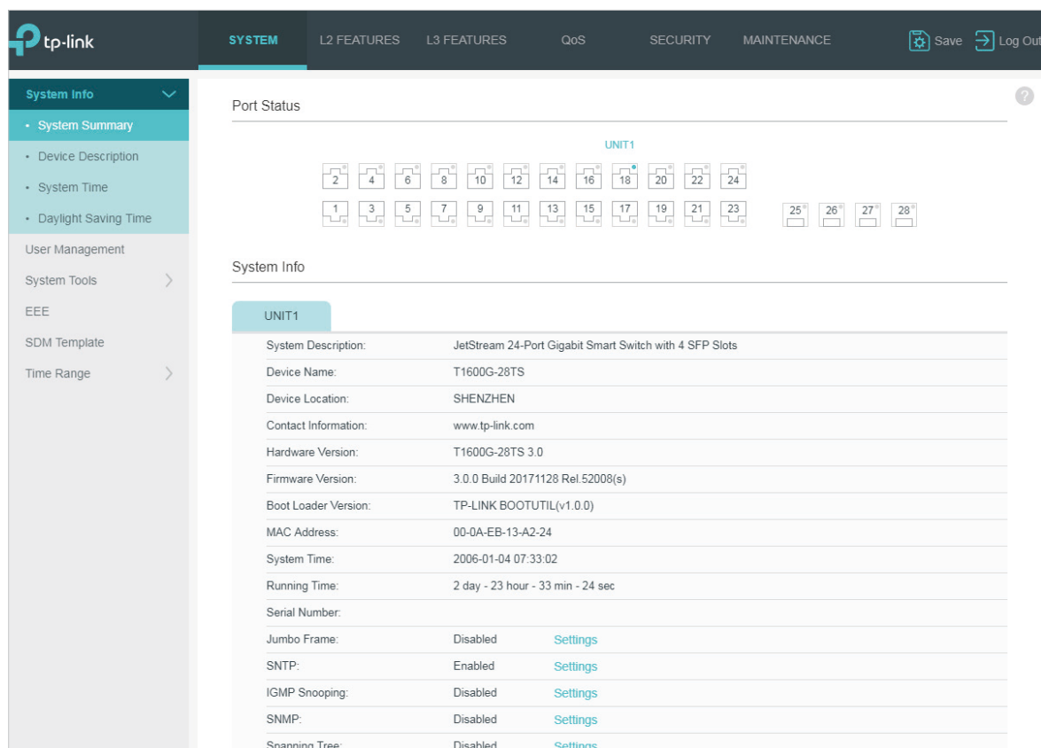
Figure 2-3 Web Interface
