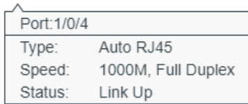
Figure 2-2 Port Information
