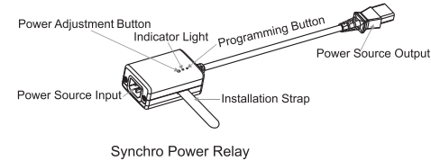
Synchro Power Relay
