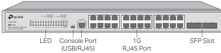
Figure 1-3 Front Panel of TL-SG3428
