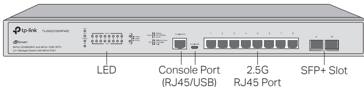
Figure 1-2 Front Panel of TL-SG3210XHP-M2
