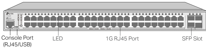
Figure 1-8 Front Panel of TL-SG3452P
