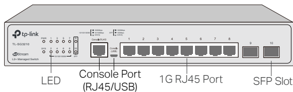
Figure 1-1 Front Panel of TL-SG3210
