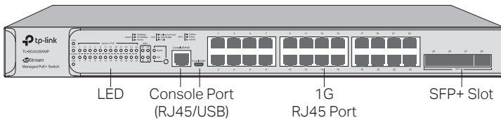
Figure 1-6 Front Panel of TL-SG3428XMP
