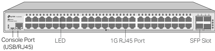
Figure 1-7 Front Panel of TL-SG3452
