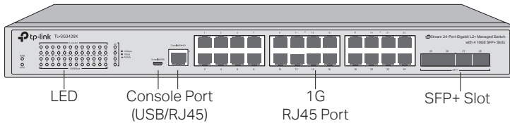
Figure 1-5 Front Panel of TL-SG3428X
