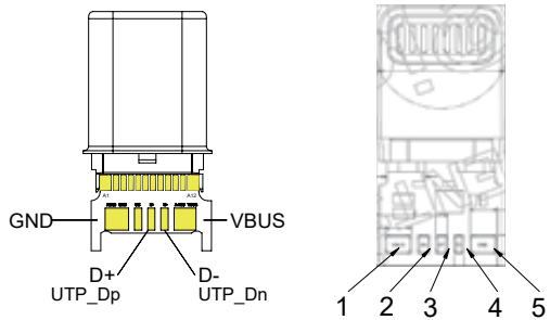
soldering view
