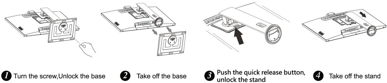
Figure.1. Installing and Removing the Base
